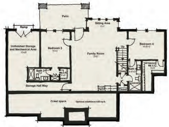
TERRACE LEVEL 1,772 SQ. FT.
